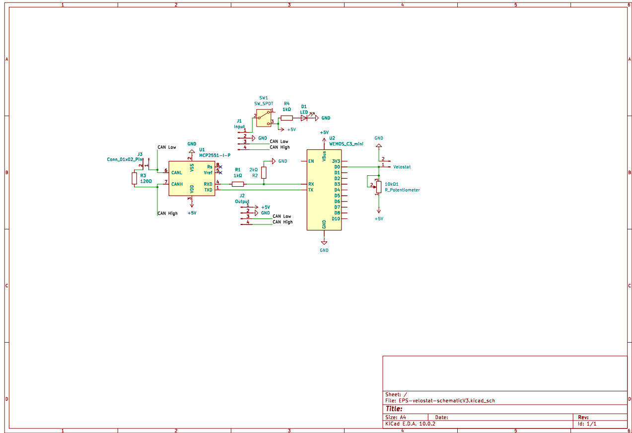
Figure 4: Central-node schematic used as the commissioning reference for CAN, power, and output wiring.
